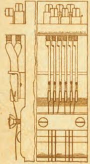
THE MASON & HAMLIN SCREW-STRINGER.
